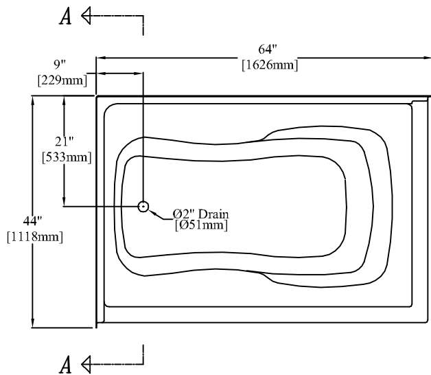
64" [1626mm] Rectangular Corner Bathtub With Removable Access Panel Left Hand Version (8864LXA) Shown
