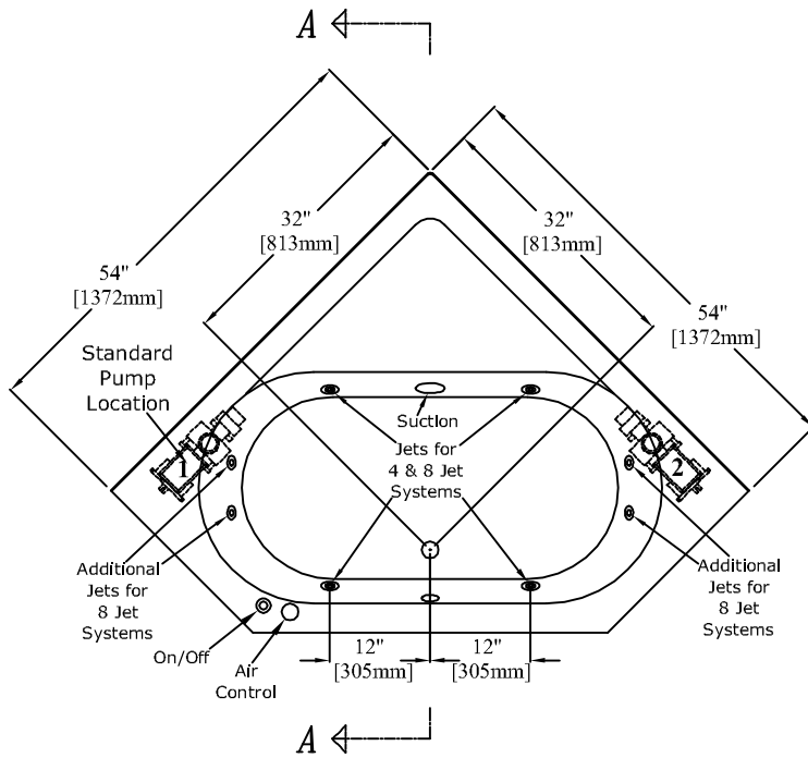
54" [1372mm] Flanged Corner Bathtub
