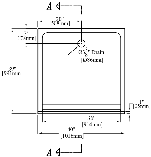
40" [1016mm] Tiled Barrier-free Shower With a 3/4" [19mm] Threshold
