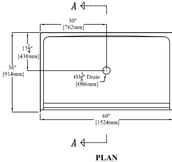
60" [1524mm] 1-Piece Barrier-free Shower Stall With 3/4" [19mm] Threshold
