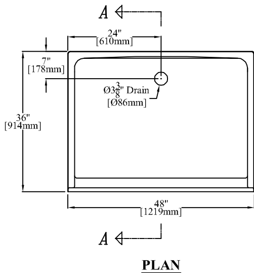
48" [1219mm] 3-Piece Barrier-free Shower Stall With 3/4" [19mm] Threshold & Rear Center Drain
