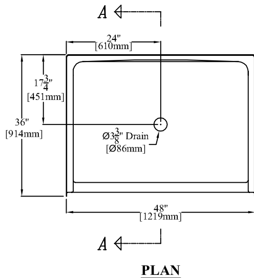
48" [1219mm] 1-Piece Barrier-free Shower Stall With 2" [51mm] Threshold
