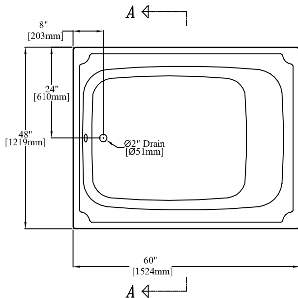
PLAN
