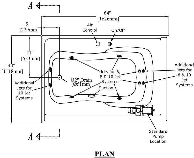
64" [1626mm] Rectangular Corner Bathtub With Removable Access Panel & 6, 8 or 10 Jet Whirlpool Package
