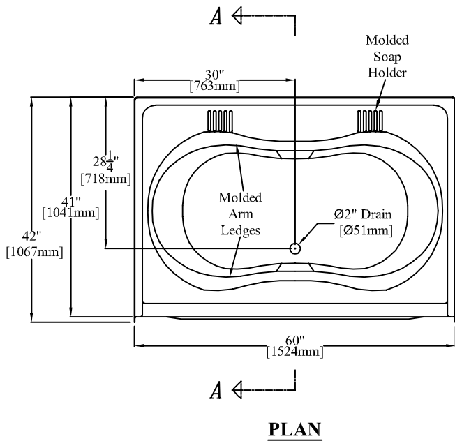
60" [1524mm] Bathtub With Removable Access Panel
