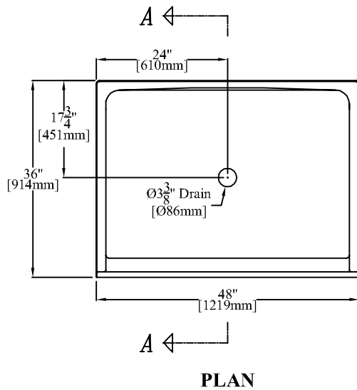
48" [1219mm] 1-Piece Barrier-free Shower Stall With 3/4" [19mm] Threshold & Center Drain
