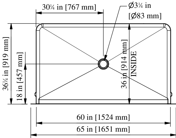
SECTION B-B 60" (65" Overall) Barrier-Free Acrylic Shower w/ 1" Threshold & Molded Dome
